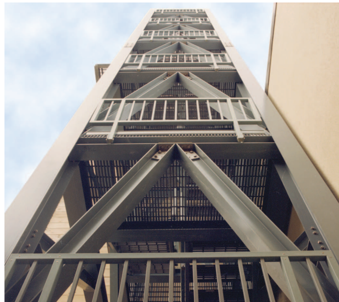
A 63' (19.2m) high freestanding fiberglass stair tower at Ft. Story Army Base, Virginia Beach, Virginia.
